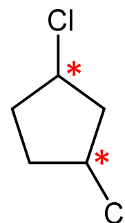
1,3-Dichlorocyclopentane
